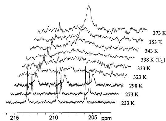
Figure 1c. Dynamic ^{13}\text{C} -NMR spectra of complex 10c in the metal carbonyl region (125 MHz, [\text{D}_8]\text{toluene} )
