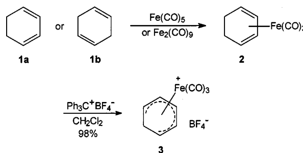
Scheme 1. Complexation of cyclohexa-1,3-diene ( 1a ) and cyclohexa-1,4-diene ( 1b ) with Fe(CO) 5 or Fe 2 (CO) 9 and preparation of the complex salt 3
