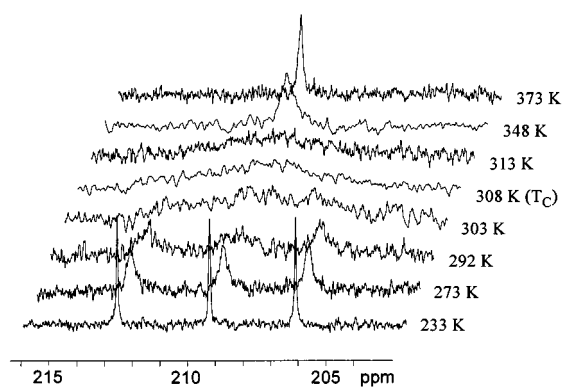
Figure 1d. Dynamic ^{13}\text{C} -NMR spectra of complex 10e in the metal carbonyl region (125 MHz, [\text{D}_8]\text{toluene} )
