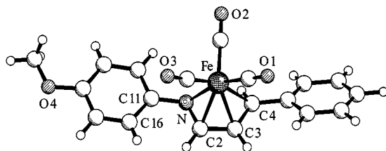
Figure 3. Molecular structure of 10c in the crystal (SCHAKAL representation; arbitrary numbering). Selected bond lengths [Å]: Fe–N 2.074(2), Fe–C2 2.064(2), Fe–C3 2.050(2), Fe–C4 2.132(3). Torsion angle: C2,N–C11,C16: 13.4°. Distance Fe–O4: 3.62 Å
