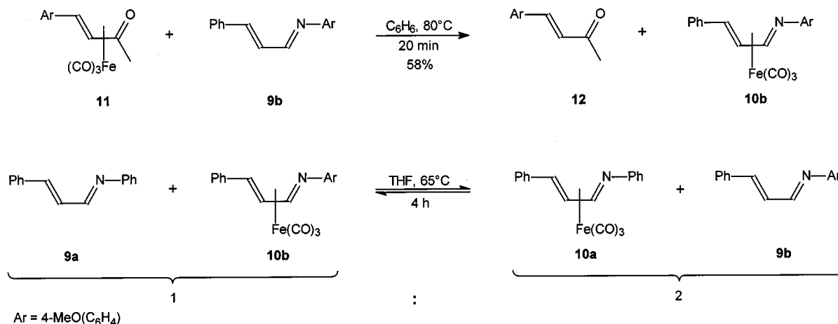
Scheme 6. Competition experiments between various tricarbonyliron transfer reagents
