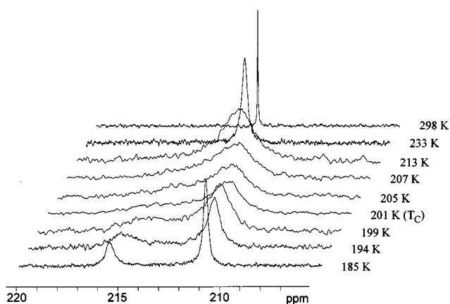
Figure 1e. Dynamic ^{13}\text{C} -NMR spectra of complex 2 in the metal carbonyl region (125 MHz, [\text{D}_8]\text{toluene} )
