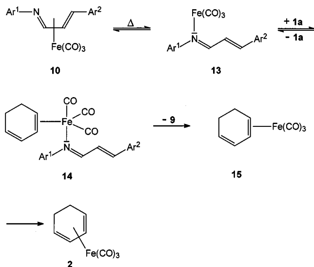
Scheme 7. Proposed mechanism of the tricarbonyliron transfer from 1,4-diaryl-1-azabuta-1,3-diene complexes 10 to cyclohexa-1,3-diene ( 1a )
