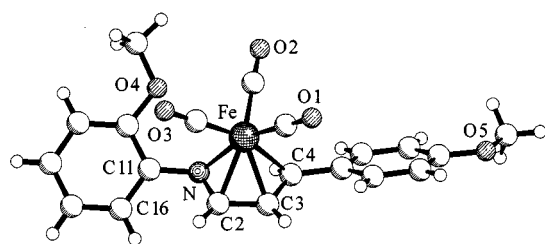
Figure 4. Molecular structure of 10l in the crystal (SCHAKAL representation; arbitrary numbering). Selected bond lengths [Å]: Fe–N 2.070(2), Fe–C2 2.068(2), Fe–C3 2.062(2), Fe–C4 2.155(2). Torsion angle: C2,N–C11,C16: 37.4°. Distance Fe–O4: 3.35 Å
