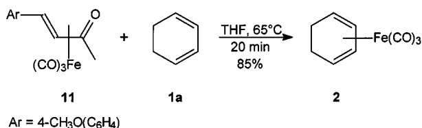
Scheme 5. Transfer of the tricarbonyliron fragment from the 4-methoxybenzylideneacetone complex 11 to cyclohexa-1,3-diene ( 1a )
