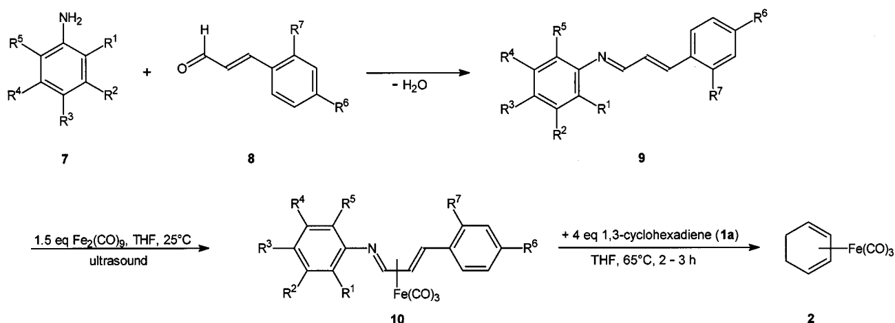
Scheme 4. Synthesis of the azadienes 9 , complexation of 9 to the iron complexes 10 with nonacarbonyldiiron, and the tricarbonyliron transfer to cyclohexa-1,3-diene ( 1a )
