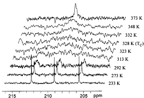
Figure 1c. Dynamic ^{13}\text{C} -NMR spectra of complex 10c in the metal carbonyl region (125 MHz, [\text{D}_8]\text{toluene} )
