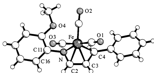
Figure 4. Molecular structure of 10l in the crystal (SCHAKAL representation; arbitrary numbering). Selected bond lengths [Å]: Fe–N 2.070(2), Fe–C2 2.068(2), Fe–C3 2.062(2), Fe–C4 2.155(2). Torsion angle: C2,N–C11,C16: 37.4°. Distance Fe–O4: 3.35 Å
